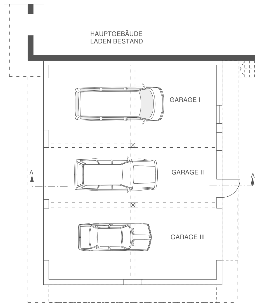
GUNDRISS ERDGESCHOSS GARAGE
